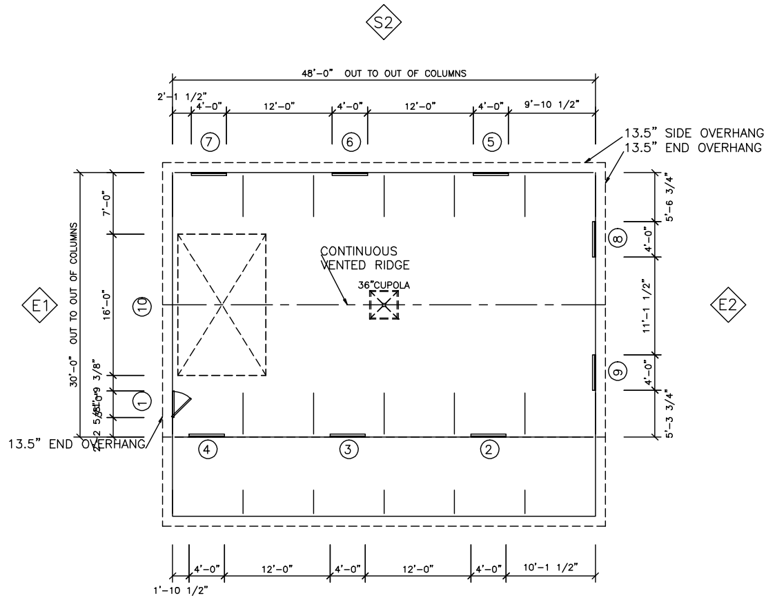
S1 Floor Plan
