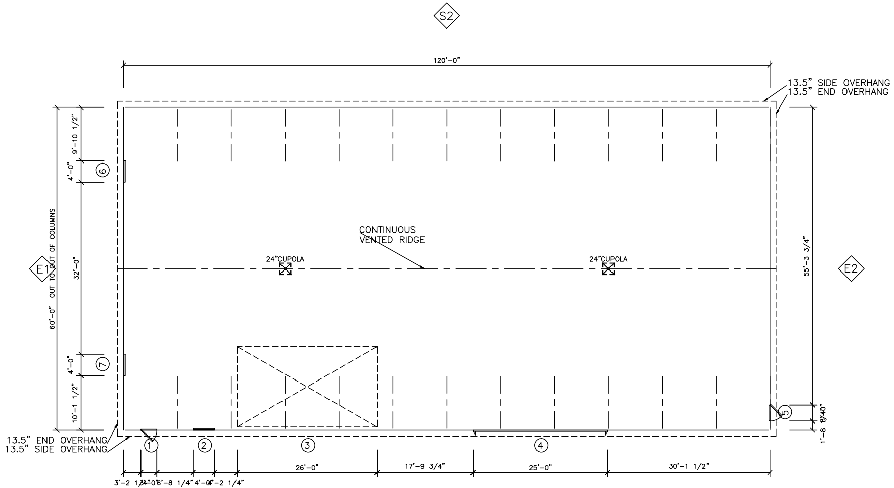
S1 Floor Plan
