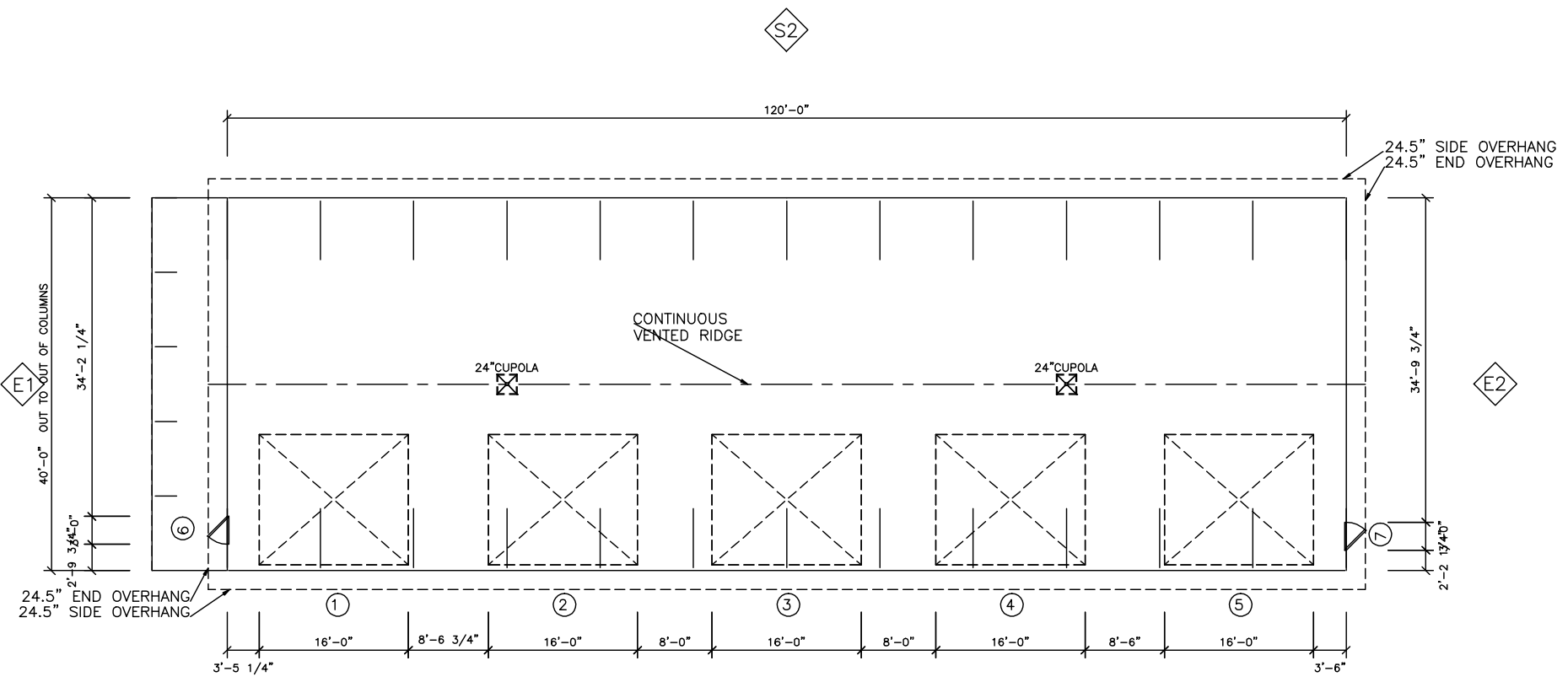
S1 Floor Plan
