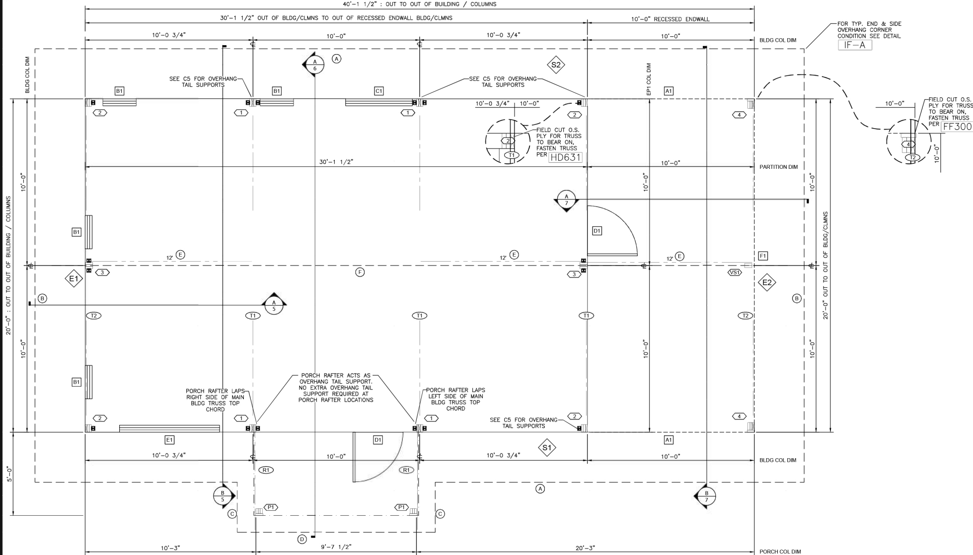
FLOOR PLAN 1/4" = 1'-0"
