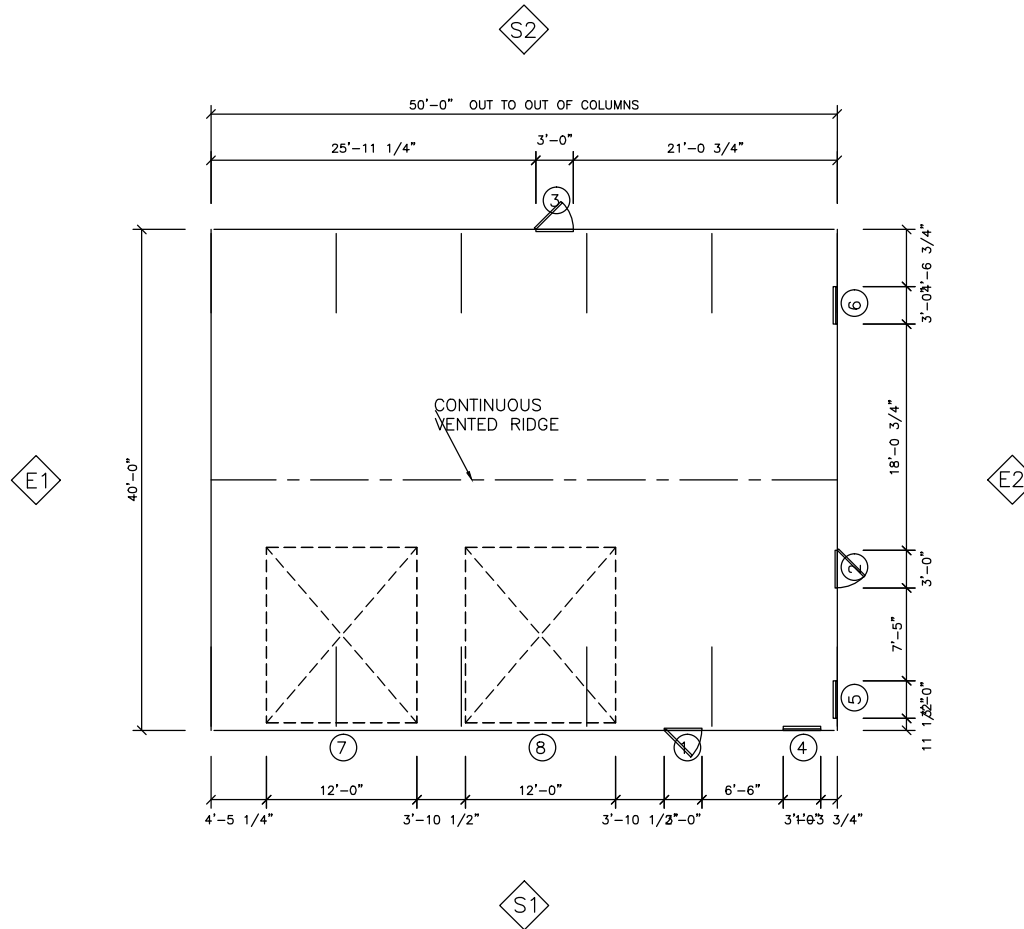
Floor Plan
