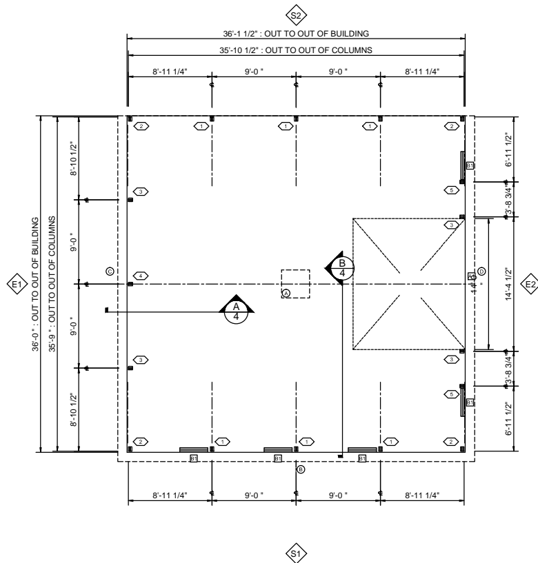
FLOOR PLAN
