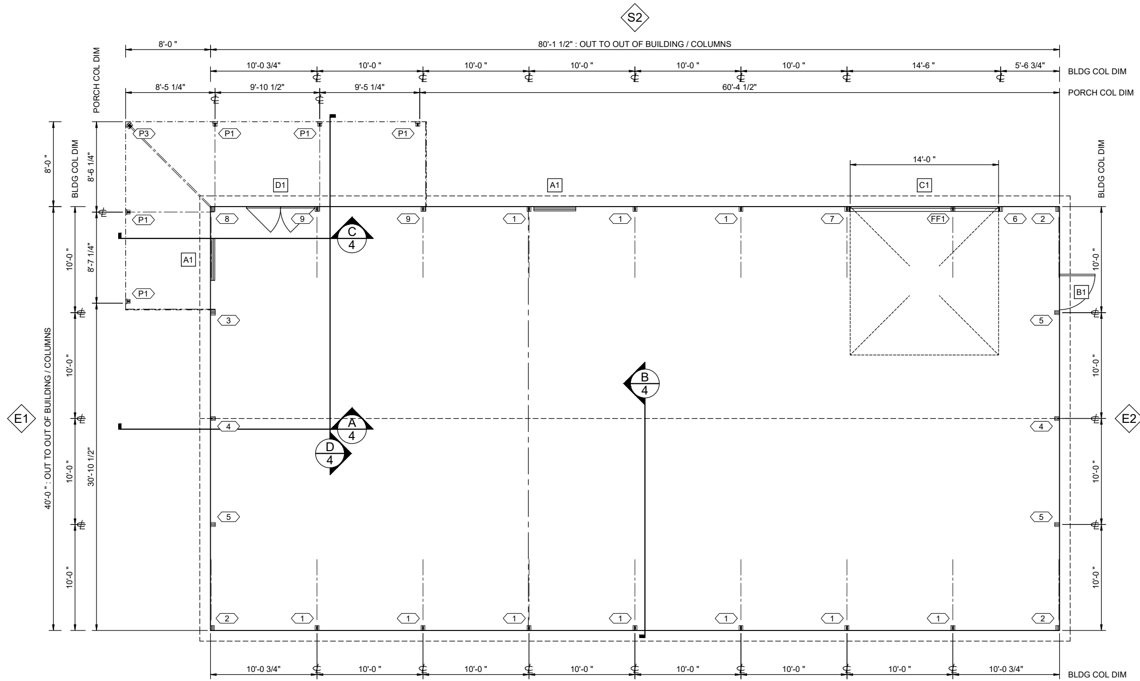
A3 FLOOR PLAN
