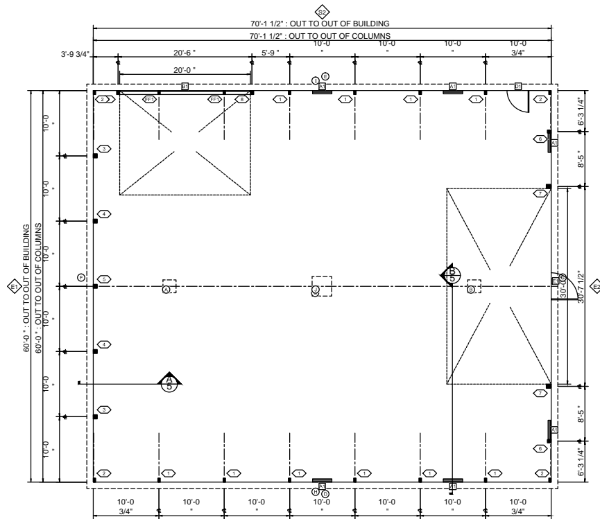
FLOOR PLAN
