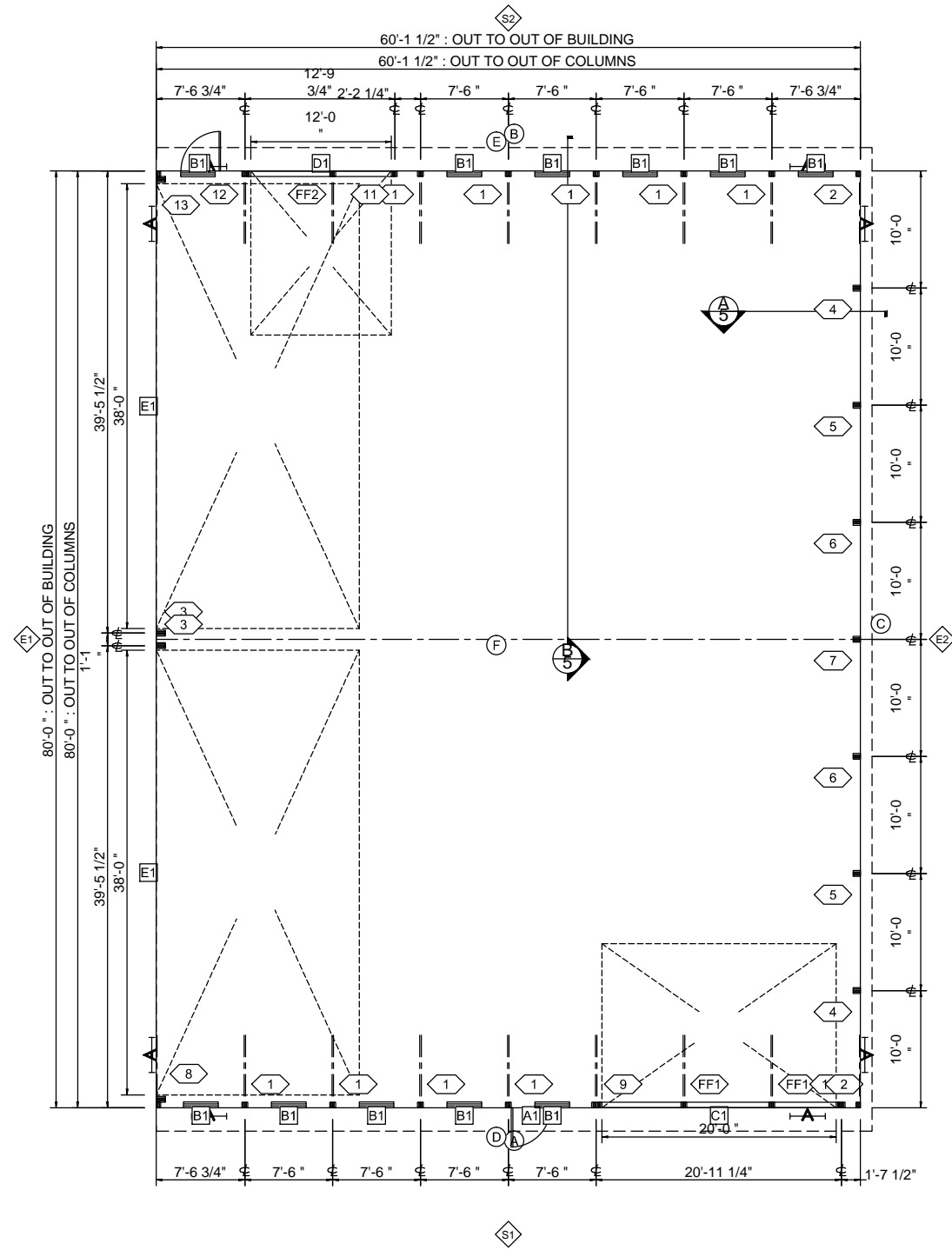
FLOOR PLAN
