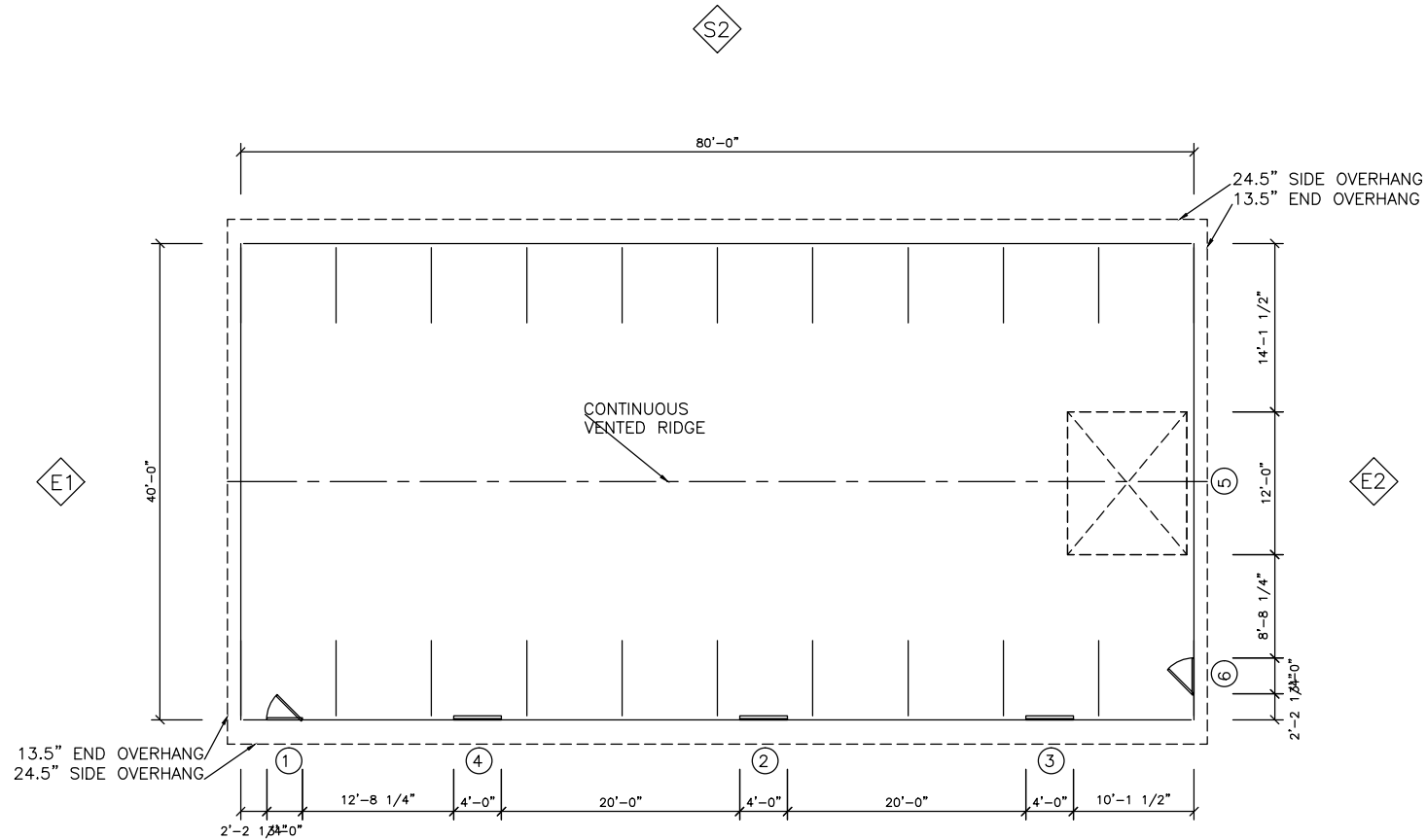
S1 Floor Plan
