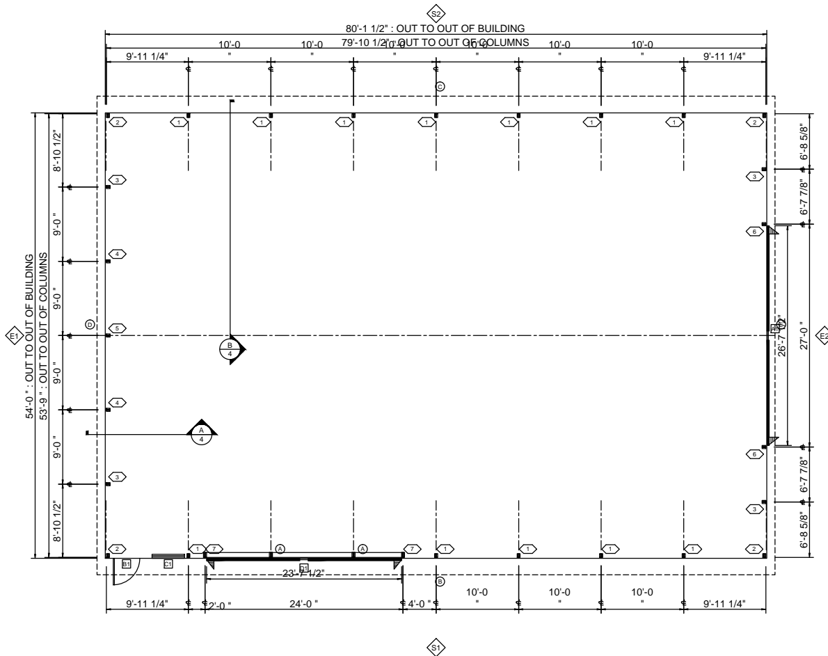
Floor Plan
