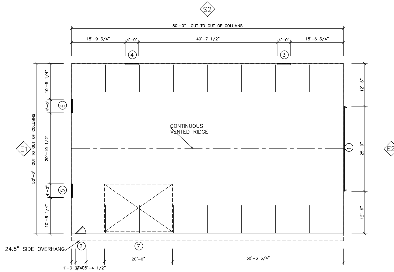
S1 Floor Plan
