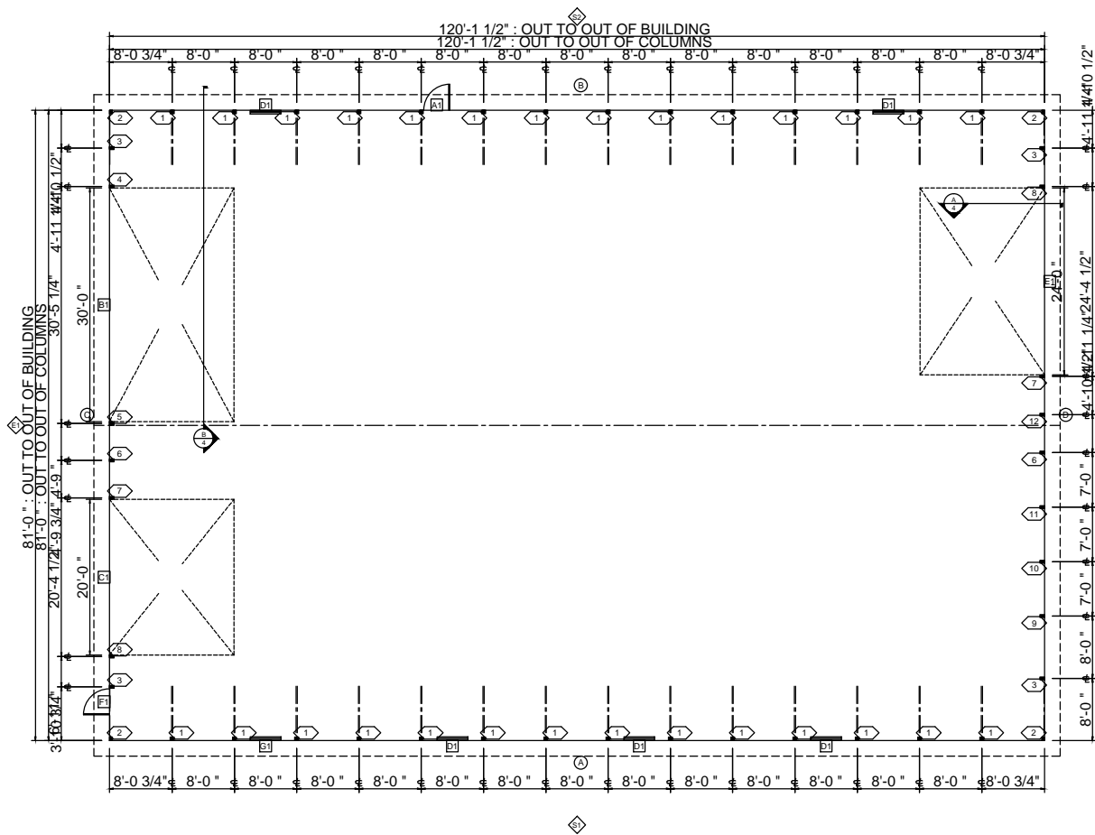
Floor Plan
