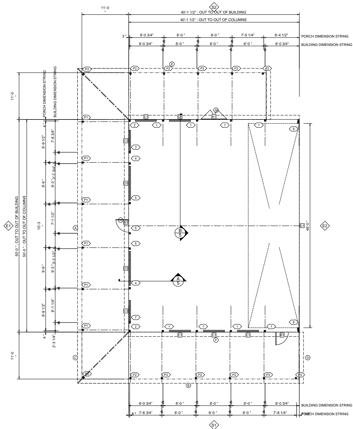
FLOOR PLAN
