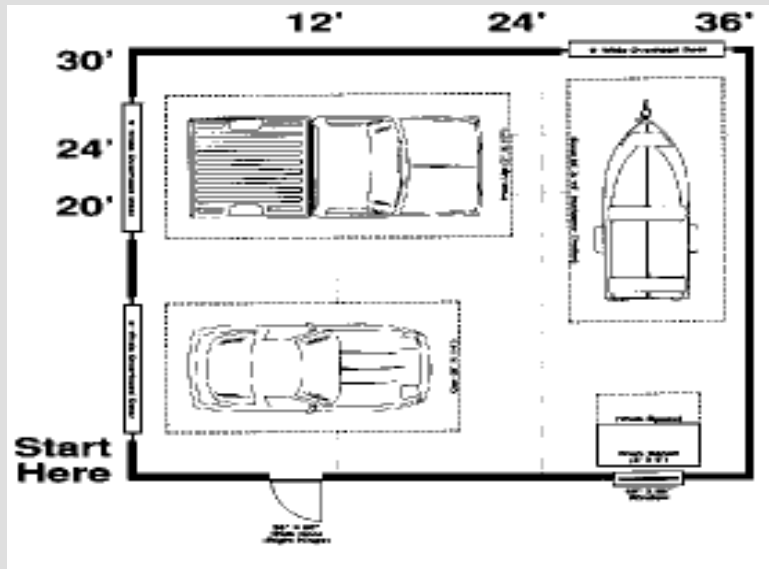
Sample of 30' x 36' Building Layout
