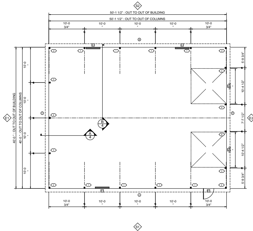
Floor Plan
