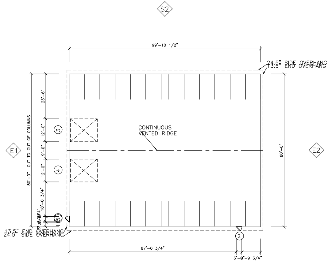
S1 Floor Plan
