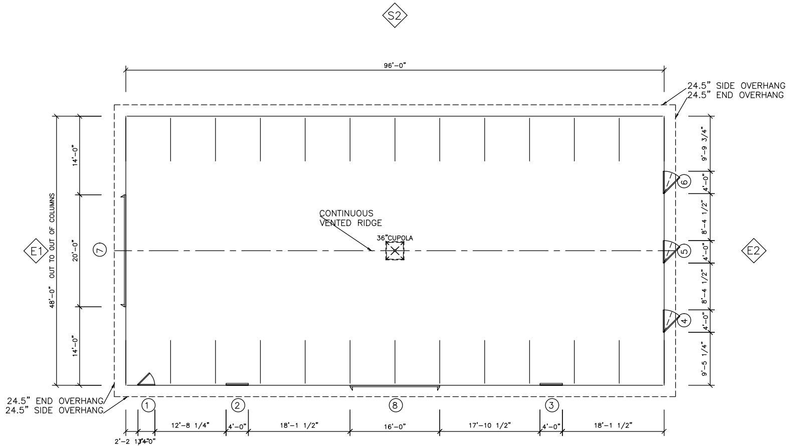
Floor Plan
