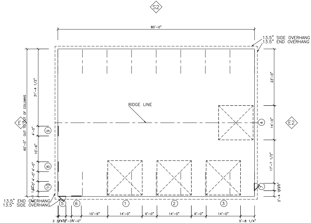
S1 Floor Plan
