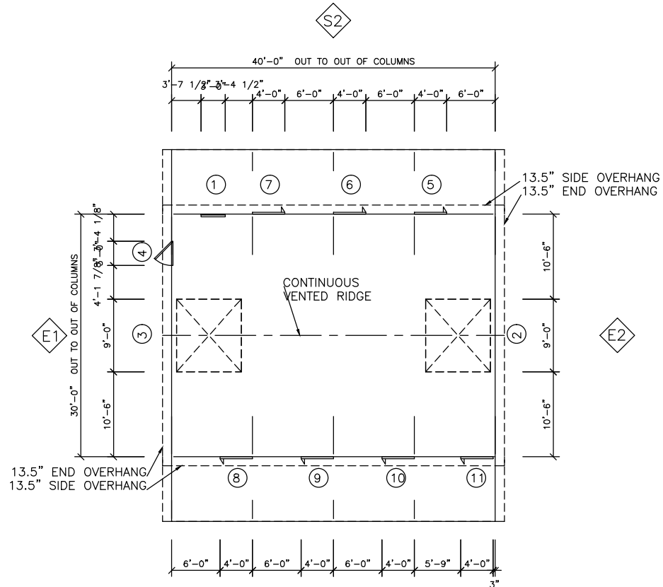
S1 Floor Plan
