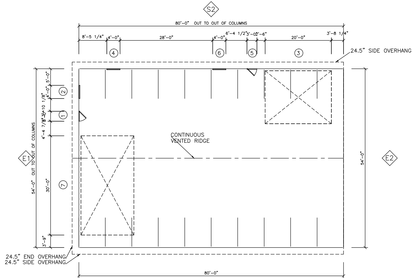
S1 Floor Plan
